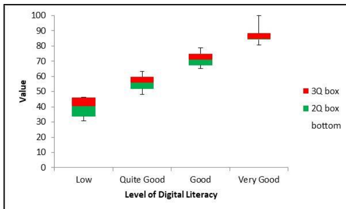
Figure 4 Students' digital literacy skills boxplot
