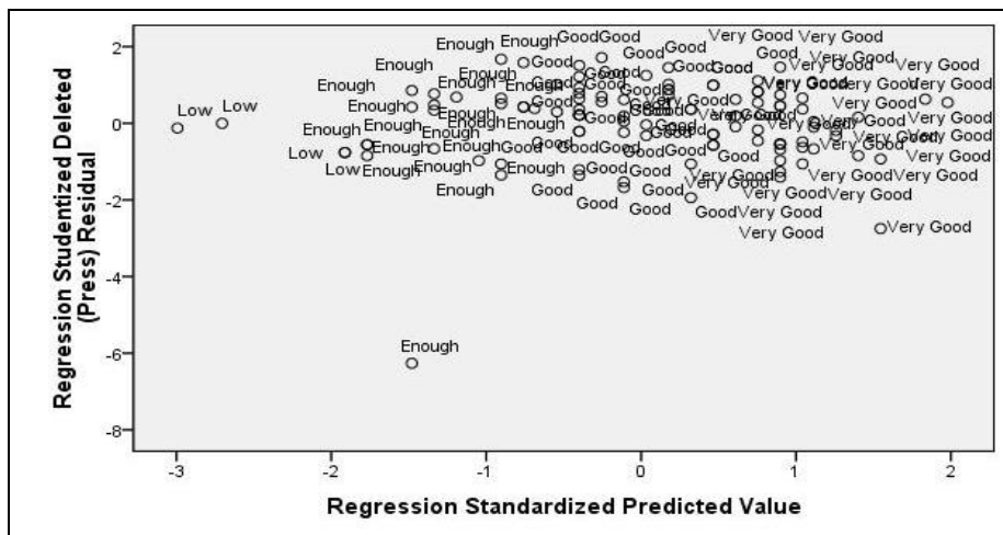
Figure 5 The scatterplot to check the feasibility of regression model
