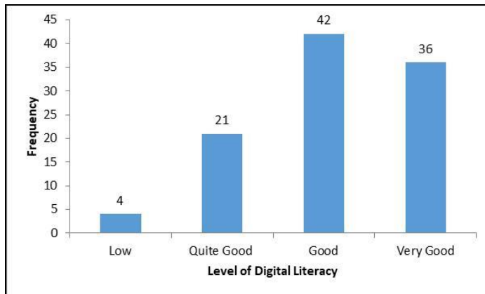
Figure 3 Students' digital literacy skills profile
